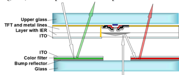
Fig. 1. Cross-section of the novel transfective LCD.
