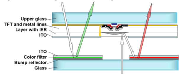
Fig. 1. Cross-section of the novel transfective LCD.
